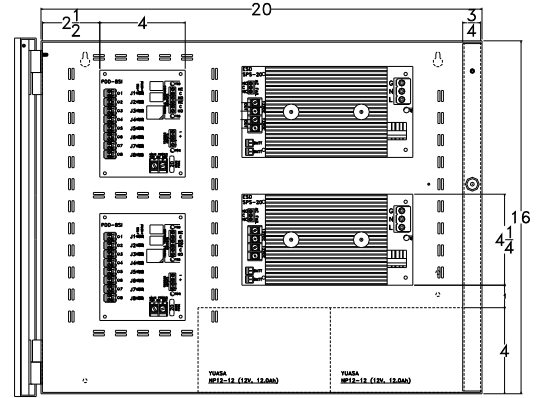
Inside dimensions / Component layout
