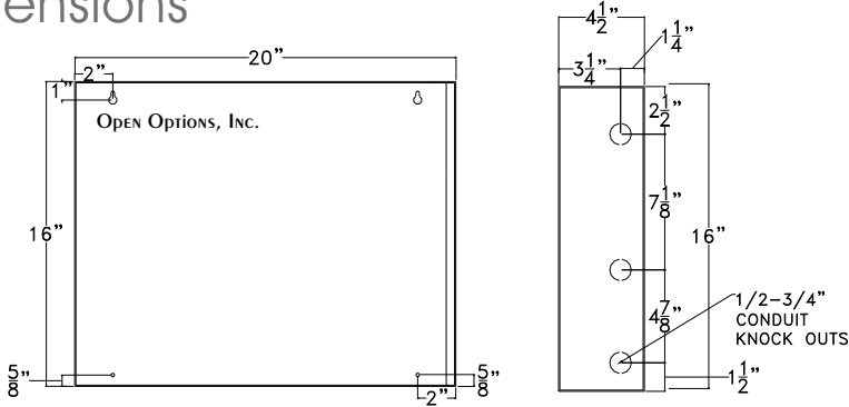
Outside dimensions / Knockout locations
